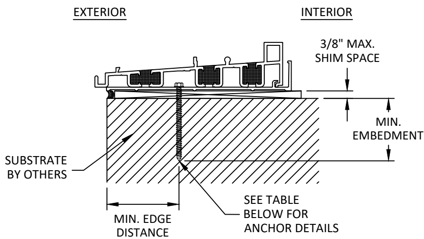
B 7 ANCHOR DETAIL LOW PROFILE SILL THROUGH FRAME NOTE: STANDARD SILL SIMILAR
