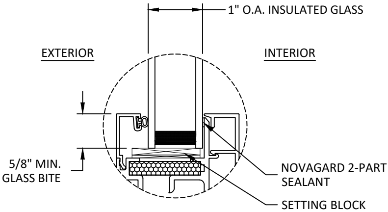
GLAZING DETAIL
